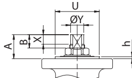
DN 250 to DN 300 (NPS 10 to NPS 12)
