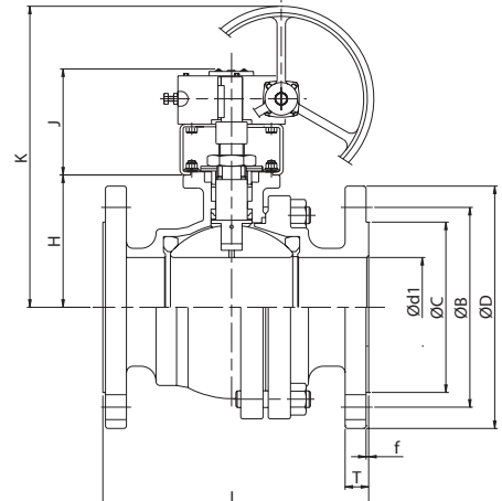
DN 250 to DN 300 (NPS 10 to NPS 12) Optional
