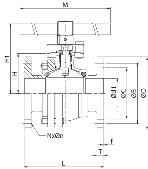
Sizes DN 65 to DN 300 (NPS 2 1/2 to NPS 12)
