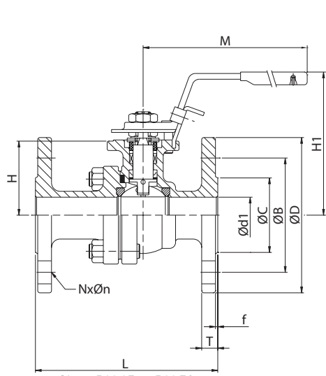
Sizes DN 15 to DN 50 (NPS 1/2 to NPS 2)
